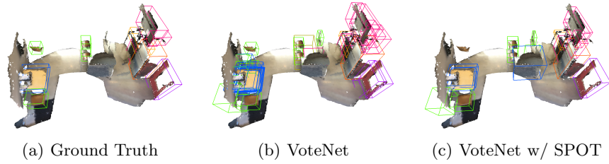
Fig. 7. Qualitative results for ScanNetV2
