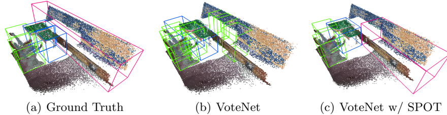
Fig. 8. Qualitative results for SUN RGB-D
