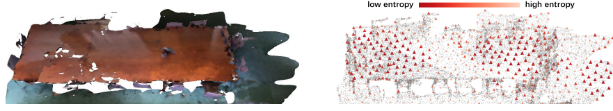
Fig. 3. Detection of suspicious coincidences. Left: A 3D scene composed of a large table. Right: Corresponding point cloud. For suspicious coincidences, the entropy of the distribution of center locations has low-entropy. These tends to happen around object regions informative for object identification and localization, such as table corners and edges.
