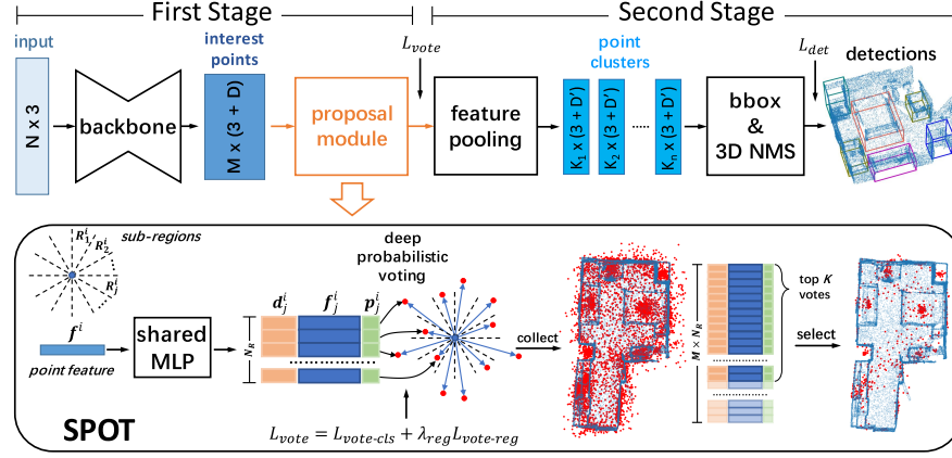
Fig. 2. Detection pipeline and Selective Point cLOUD voTing (SPOT). The proposal module of existing point cloud detectors is replaced by the proposed SPOT for better localization of object centers.
