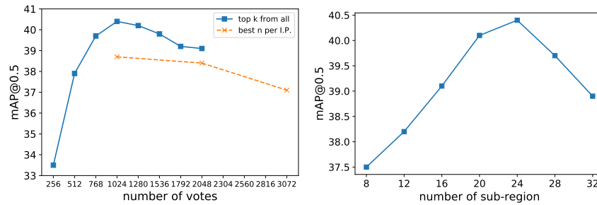
Fig. 4. Analysis of number of votes and sub-regions. Left: Number of votes v.s. mAP performance, under the case of 24 sub-regions. Right: Number of sub-regions v.s. mAP performance, under the case of 1024 votes.
