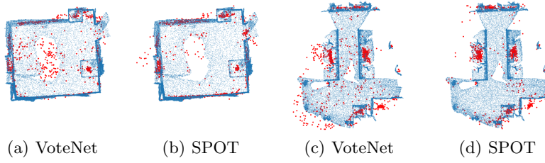
Fig. 5. Votes from baseline model and SPOT. Red dots are center votes.
