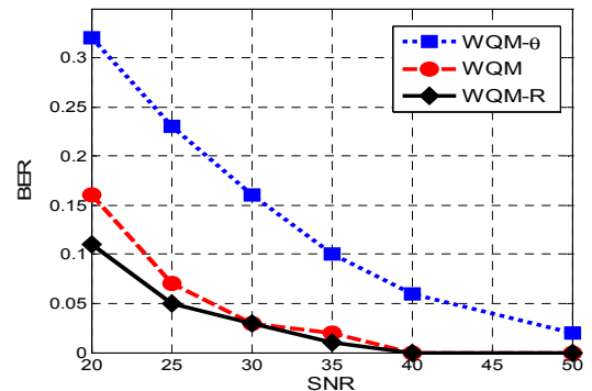
Fig. 2. BER of the proposed methods for 0.25 bps
